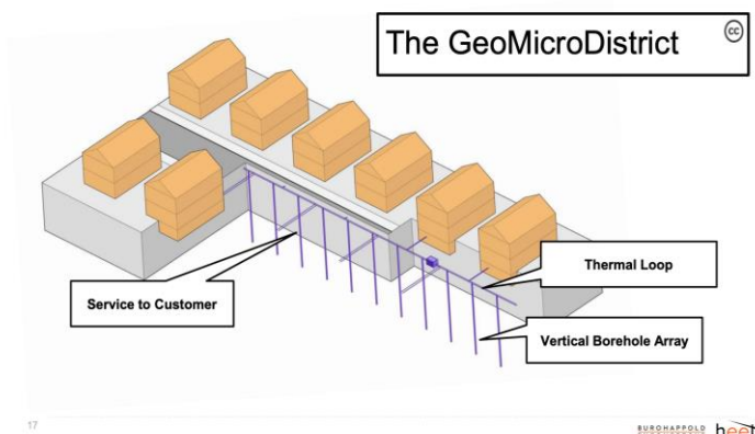
FIGURE 3: UTILITY-SCALE NETWORKED GROUND-SOURCE HEAT PUMPS: GEOMICRODISTRICT 80
